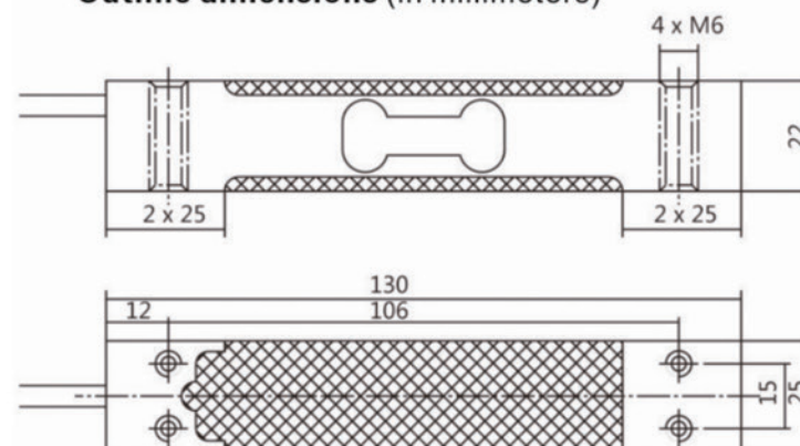
Outline dimensions (in millimeters)
